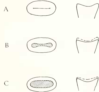
TEXT-FIG. 2. Procolophon trigoniceps . Stages of tooth wear, worn surfaces on the left, sectional views on the right, with previous wear stage shown by dashed line. A, points connected by a sharp ridge. B, wear on the points slower as greater cross-sectional area is exposed. C, stage of uniform wear.
